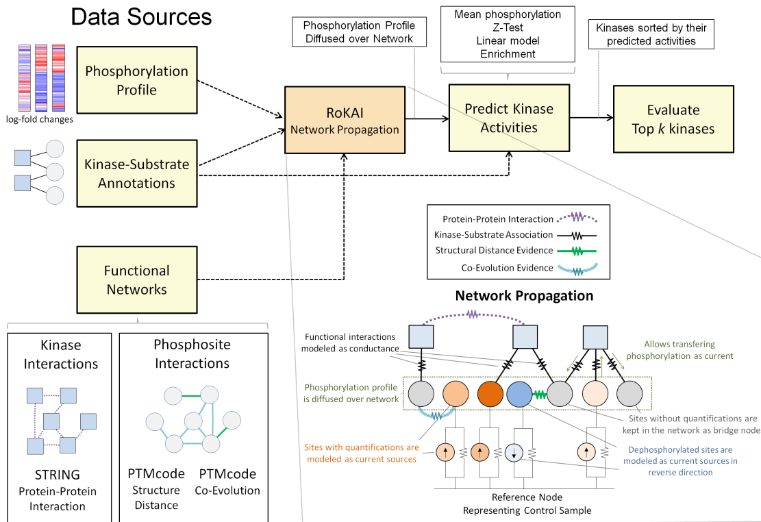
Figure 1. The workflow and the key idea of RoKAI. Traditional algorithms for kinase activity inference use condition-specific phosphorylation data and available kinase-substrate associations to identify kinases with differential activity in each condition. RoKAI integrates functional networks of kinases and phosphorylation sites to generate robust phosphorylation profiles. The network propagation algorithm implemented by RoKAI ensures that unidentified sites that lack quantification levels in a condition can still be used as bridges to propagate phosphorylation data through functional paths.
